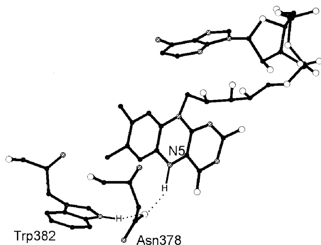
FIGURE 1: Conformations of the FAD cofactor and vicinal residues Asn378 and Trp382 in E. coli DNA photolyase.
