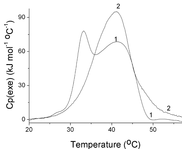
FIGURE 3: DSC thermograms of the N378S mutant protein in the oxidized form at 40 \mu M (trace 1) and the dithionite-reduced sample at 28 \mu M (trace 2). The scan rates were 1 ^{\circ} C/min.
