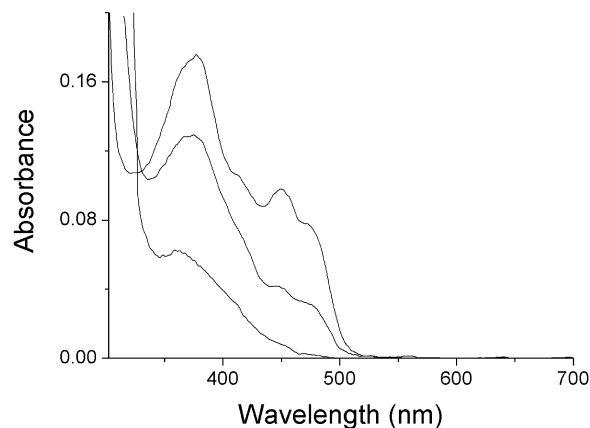
FIGURE 4: Photoreduction of N378S mutant photolyase. During photoreduction, the 380 nm peak and the 450 nm peak of the mutant protein decreased in magnitude and only a broad peak at 360 nm was left finally.
